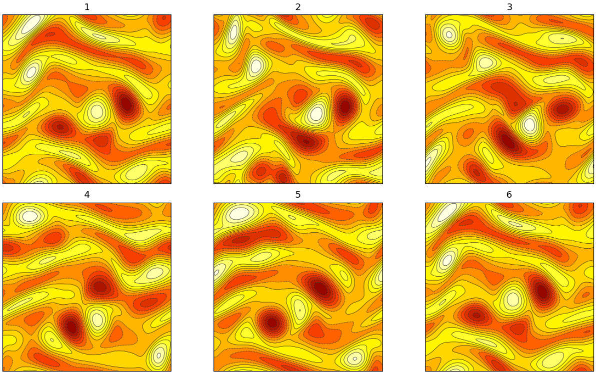
Figure 4.11: Vorticity-field snapshots of the relative periodic orbit R_3 at times 0, 1.19, 2.39, 3.58, 4.60, 5.60, shown using 15 contour levels, with -9.56 \leq \omega \leq 7.44 . Darker shades indicate negative vorticity, while lighter shades indicate positive vorticity.
